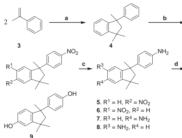
Scheme 1. (a) TFA, rt 12 h; (b) HNO 3 /(Ac) 2 O, 0 °C, 4 h; (c) Pd/C, hydrazine, reflux, 4 h; (d) H 2 SO 4 , NaNO 2 , H 2 O, 0 °C/heat.
