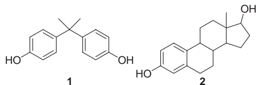
Chart 1. Chemical structures for bisphenol A (1) and 17 \beta -estradiol (2).
