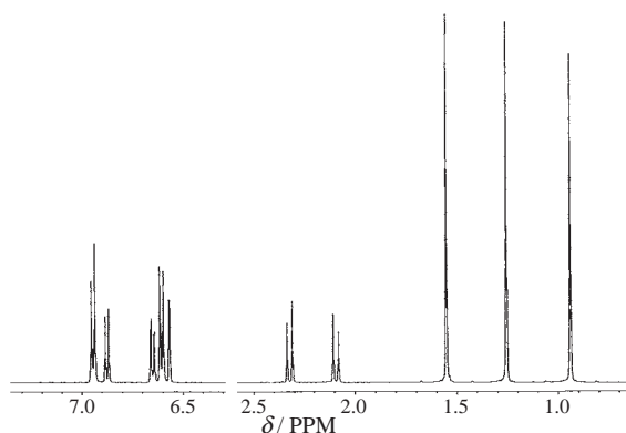
Figure 1. 1 H NMR spectra of 5-hydroxy-1-(4'-hydroxyphenyl)-1,3,3-trimethylindan ( 9 ).
